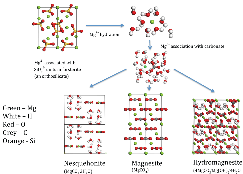
Figure 1. Possible reaction paths in the transformation of an orthosilicate mineral (forsterite) to possible magnesium carbonate minerals in the presence of CO 2 . The reaction path involves the dissolution of Mg 2+ from the forsterite surface, hydration and/or carbonation of the Mg 2+ ion in solution, followed by the precipitation of magnesium carbonate mineral phases depending on the dynamics of the transformation.
